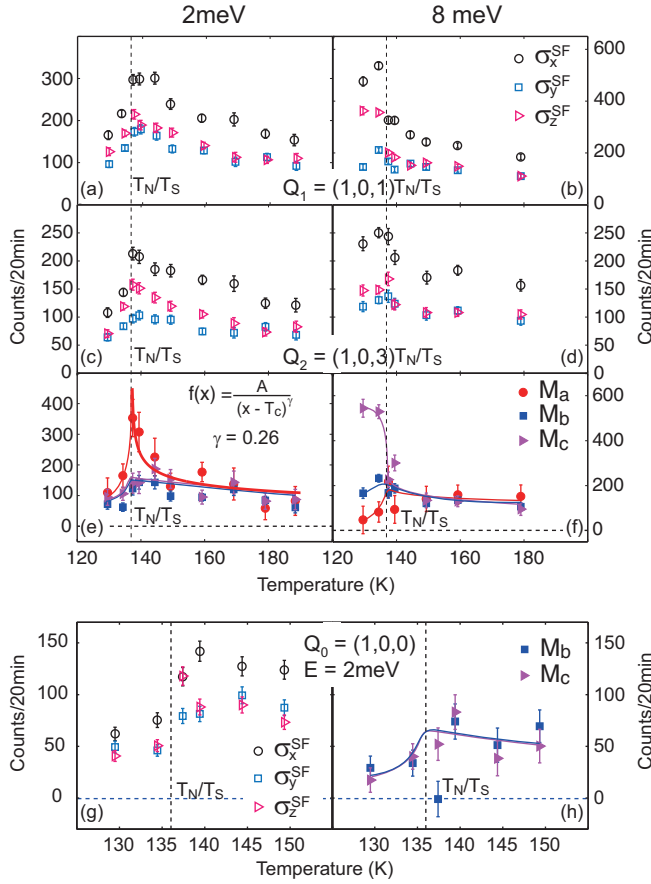
FIG. 4. Temperature dependence of \sigma_x^{\text{SF}} , \sigma_y^{\text{SF}} , and \sigma_z^{\text{SF}} at E = 2 meV with (a) \mathbf{Q}_1 = (1,0,1) and (c) \mathbf{Q}_2 = (1,0,3) . Similar data at E = 8 meV with (b) \mathbf{Q}_1 = (1,0,1) and (d) \mathbf{Q}_2 = (1,0,3) . (e) Temperature dependence of the components M_a , M_b , and M_c at E = 2 meV. The solid curve is the fitted line with function f(T) = \frac{A}{(T - T_c)^\gamma} . (f) Temperature dependence of M_a , M_b , and M_c at E = 8 meV. (g) The three SF scattering channels measured at \mathbf{Q}_0 = (1,0,0) and E = 2 meV. (h) Temperature dependence of M_b and M_c determined from (g). The solid lines are guides to the eye. The vertical dashed lines mark T_N/T_s .
