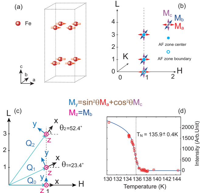
FIG. 1. (a) The orthorhombic unit cell of \text{BaFe}_2\text{As}_2 (enclosed by dashed line) with only the magnetic Fe ions shown as red spheres. The arrows indicate the ordered moment direction along the longer a axis. Along the c axis the nearest neighboring spins are antiparallel. (b) The positions of reciprocal space probed in the present experiment. Magnetic fluctuations polarized along the a , b , and c directions are marked as M_a , M_b , and M_c , respectively. (c) Schematic of the [H, 0, L] scattering plane, where wave vectors \mathbf{Q}_0 , \mathbf{Q}_1 , and \mathbf{Q}_2 are probed. The neutron polarization directions are along the x , y , and z . The angle between the x direction and H axis is denoted as \theta . (d) The temperature dependence of magnetic order parameter measured at \mathbf{Q}_1 = (1, 0, 1) . The solid line is a Gaussian convolved power law fit with T_N = 135.9 \pm 0.4 K.
