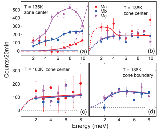
FIG. 3. (a–c) The magnetic components M_a , M_b , and M_c at \mathbf{Q}_{\text{AF}} and 135 , 138 , and 160 K obtained from data in Fig. 2. The dashed lines in (a) are results for spin waves of \text{BaFe}_2\text{As}_2 at 2 K [21]. (d) The magnetic components at the zone boundary (ZB) at 138 K. Only M_b and M_c can be determined from measurements at \mathbf{Q} = (1, 0, 0) .
