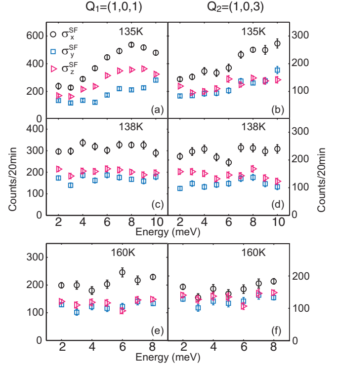
FIG. 2. Constant- \mathbf{Q} scans at the two AF wave vectors \mathbf{Q}_1 = (1, 0, 1) and \mathbf{Q}_2 = (1, 0, 3) at T = 135 , 138 , and 160 K. All three spin-flip (SF) channels \sigma_x^{\text{SF}} , \sigma_y^{\text{SF}} , \sigma_z^{\text{SF}} are measured at these wave vectors as defined in Fig. 1(c).
