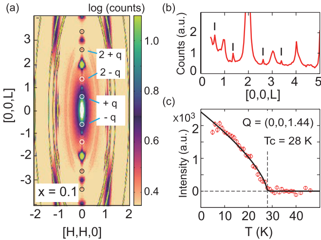
FIG. 7. (a) Neutron diffraction measurements on \text{Sr}(\text{Co}_{0.9}\text{Ni}_{0.1})_2\text{As}_2 in the [H, H, L] plane [24]. (b) One-dimensional cut along the [0, 0, L] direction in (a). The intensities at (0, 0, L) with L being an odd number are due to double scattering [34]. (c) Temperature dependence of the magnetic peak at Q = (0, 0, 1.44) .
