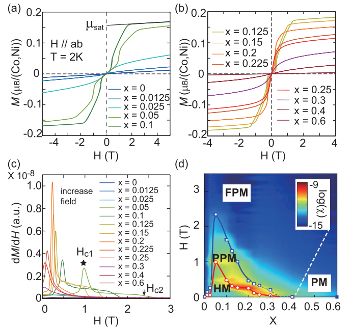
FIG. 3. (a) and (b) M(H) for crystals with 0 \leq x \leq 0.6 . (c) dM/dH vs H for 0 \leq x \leq 0.6 . (d) Magnetic phase diagram with H and x . H_{c1} and H_{c2} are defined in (c). H_{c2} is represented by the blue dashed curve where it is poorly determined by the data. The white dashed line is a speculative separation (or crossover) between paramagnetic (PM) and field-induced FM states. PPM refers to the partially polarized magnetic state, and FPM means the fully polarized magnetic state.
