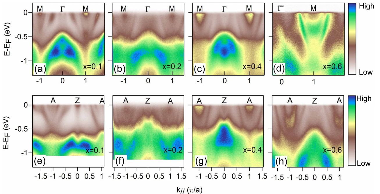
FIG. 10. Intensity plots of the band dispersion along (a)–(d) the \Gamma - M and (e)–(h) Z - A directions from ARPES measurements for x = 0.1, 0.2, 0.4, and 0.6 .
