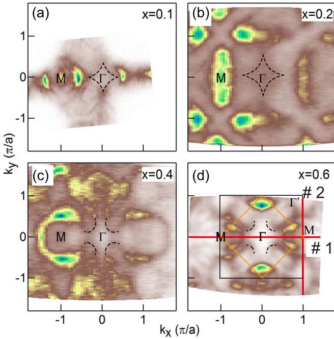
FIG. 9. Plot of the ARPES intensity at E_F of \text{Sr}(\text{Co}_{1-x}\text{Ni}_x)_2\text{As}_2 with x = 0.1, 0.2, 0.4, and 0.6 . A complex structure of Fermi surfaces is observed, and the topology changes dramatically from x = 0.1 to x = 0.6 due to the existence of flat-band dispersion. The dashed lines are a guide to the eye.
