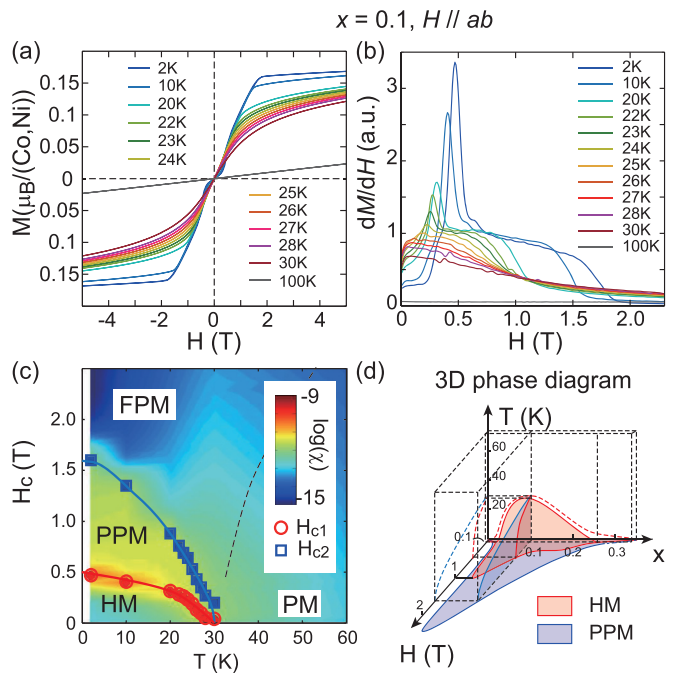
FIG. 5. (a) and (b) M_{ab} and dM_{ab}/dH vs H at temperatures identified in the plots. (c) Phase diagram determined from data in (a) and (b). The dashed line is a speculative crossover separating the fully polarized magnetic (FPM) and paramagnetic (PM) phases. PPM denotes the partially polarized magnetic phase. (d) Three-dimensional phase diagram combining Figs. 2(d), 3(d), and 7(c).
